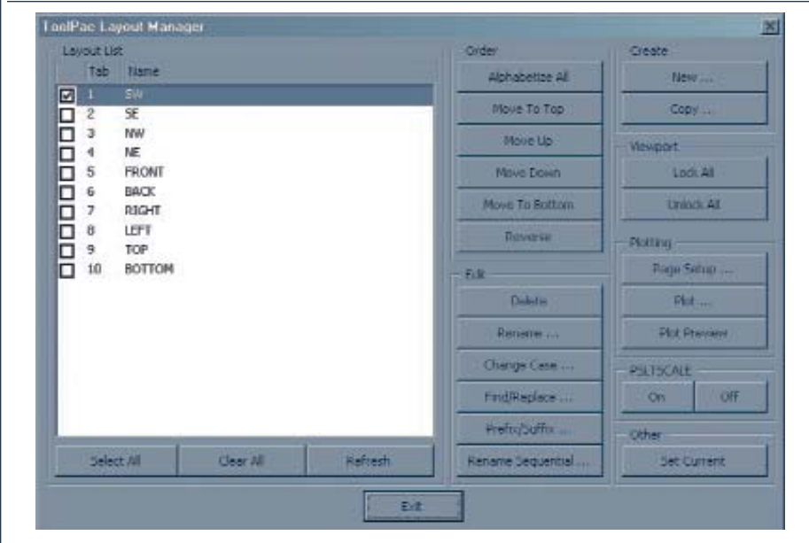
Figure 5. Layout Manager Dialog Box
